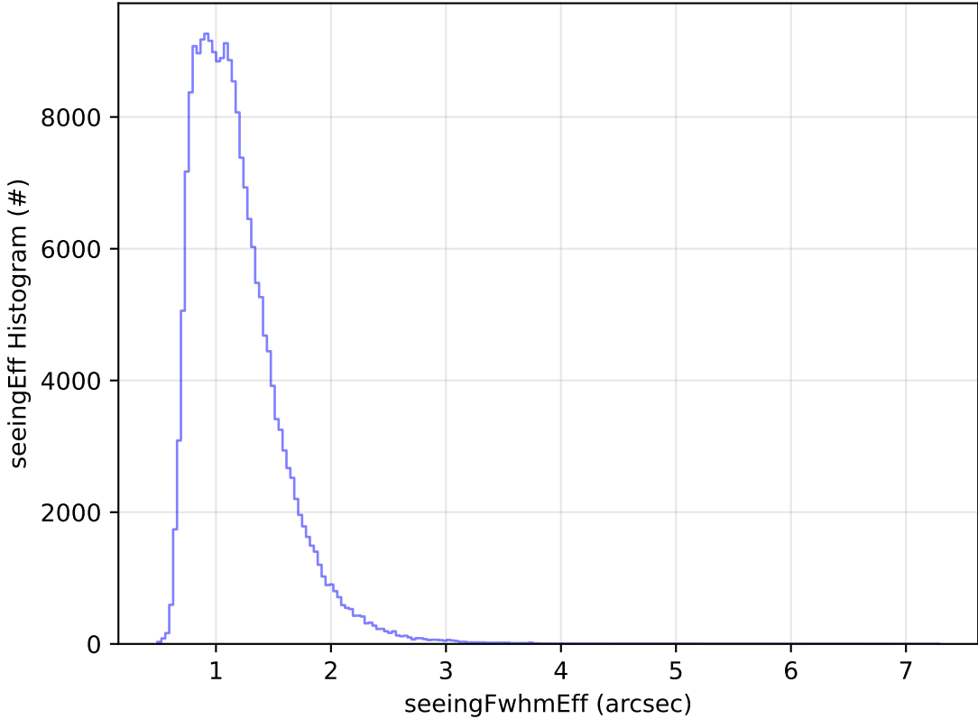
weather_cloudso0v3.5_10yrs WFD g band: seeingEff Histogram
