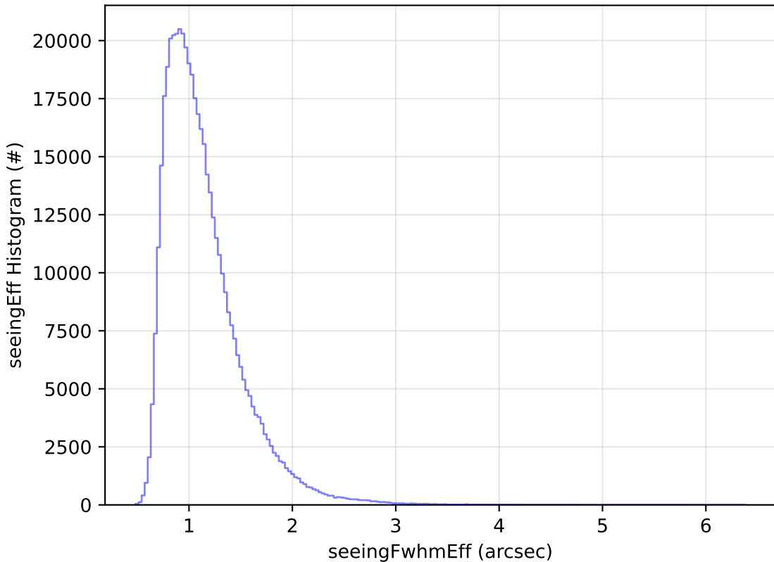
weather_cloudso0v3.5_10yrs All sky r band: seeingEff Histogram
