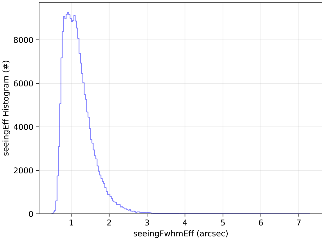
weather_cloudso0v3.5_10yrs All sky g band: seeingEff Histogram
