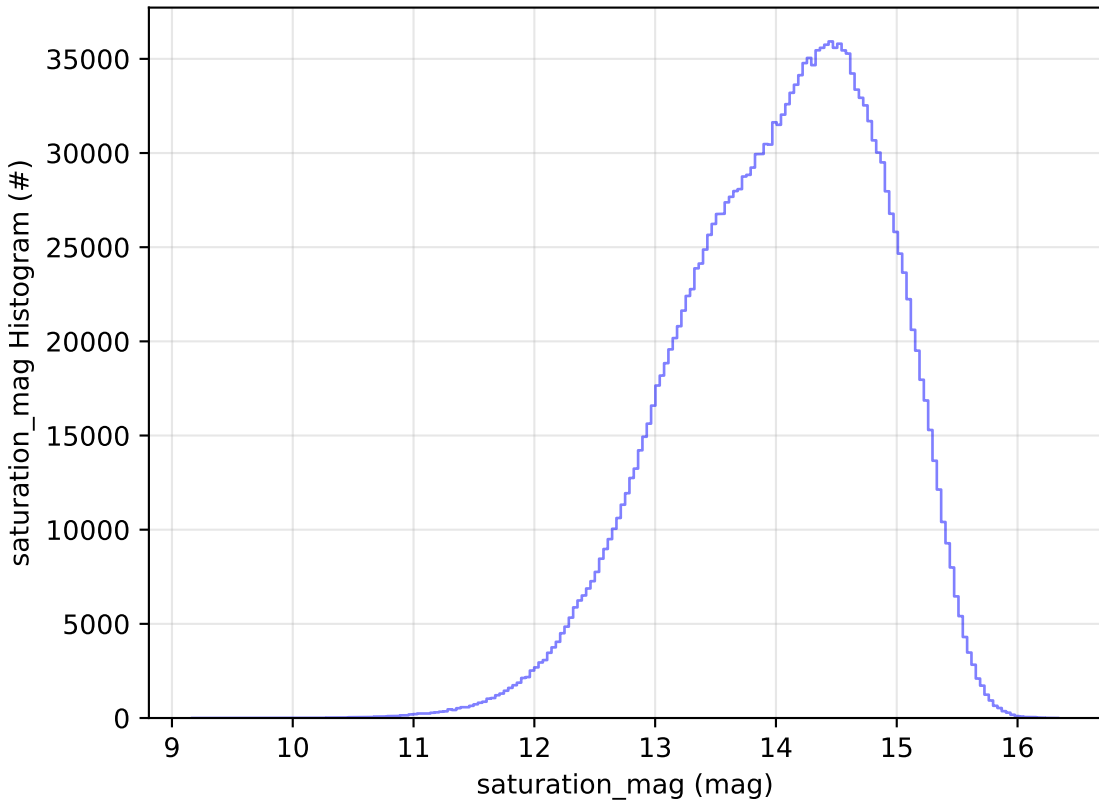
weather_cloudso0v3.5_10yrs WFD all bands: saturation_mag Histogram
