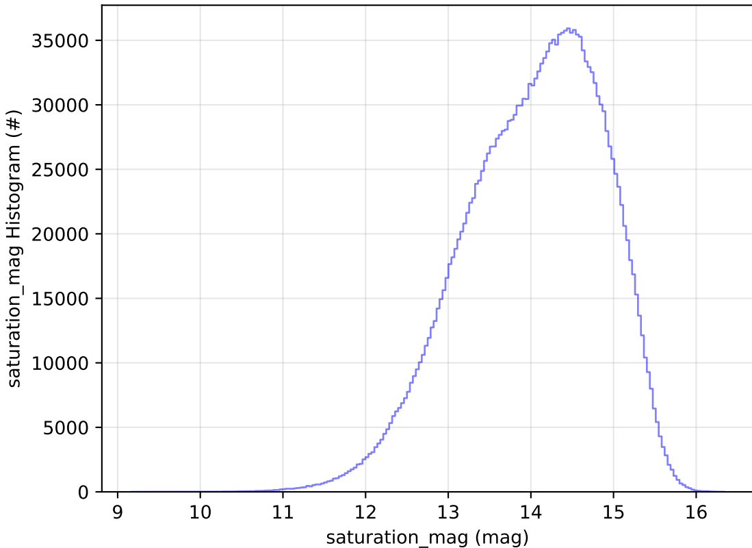
weather_cloudso0v3.5_10yrs All sky all bands: saturation_mag Histogram
