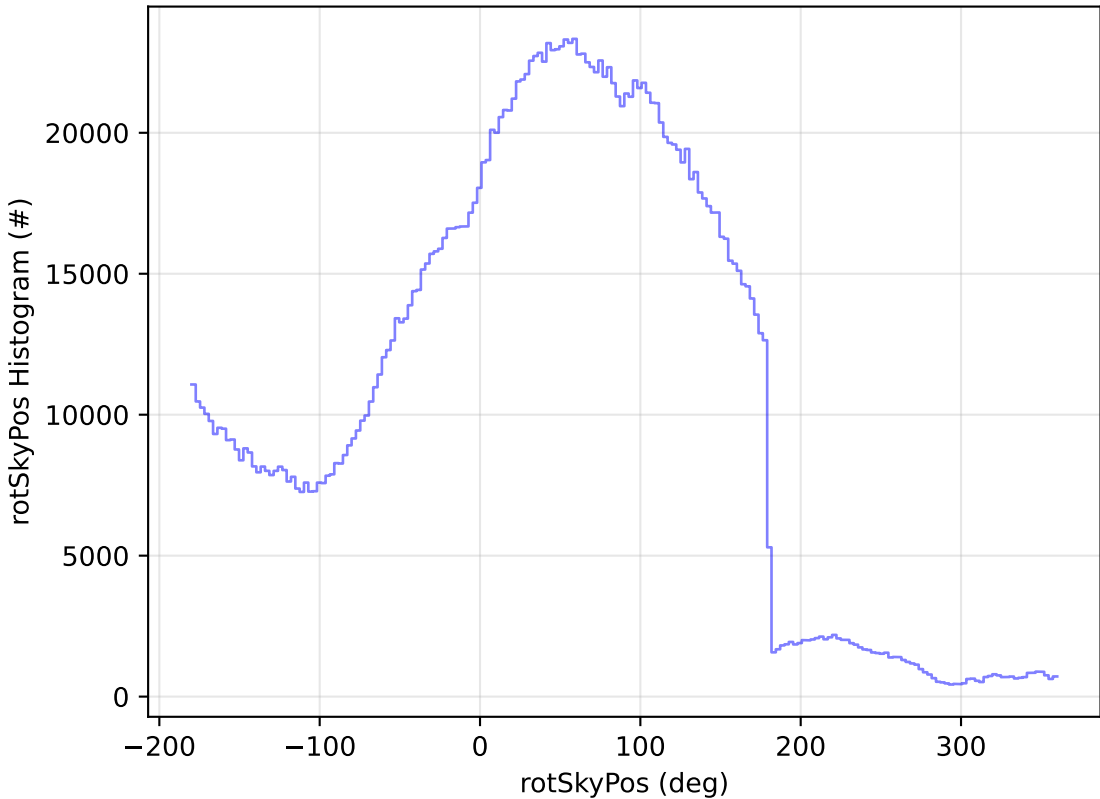
weather_cloudso0v3.5_10yrs WFD all bands: rotSkyPos Histogram
