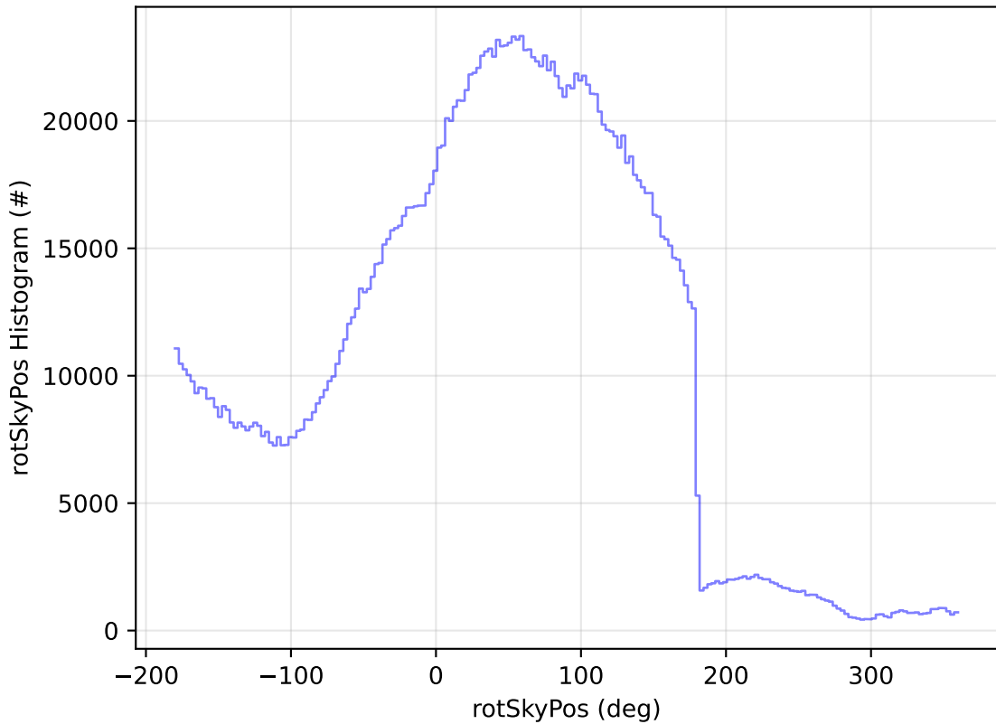
weather_cloudso0v3.5_10yrs All sky all bands: rotSkyPos Histogram
