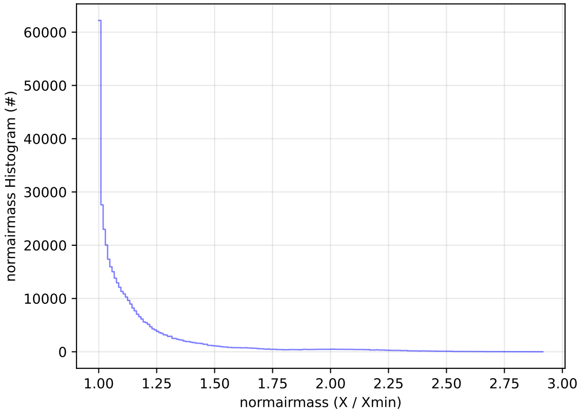
weather_cloudso0v3.5_10yrs WFD z band: normairmass Histogram
