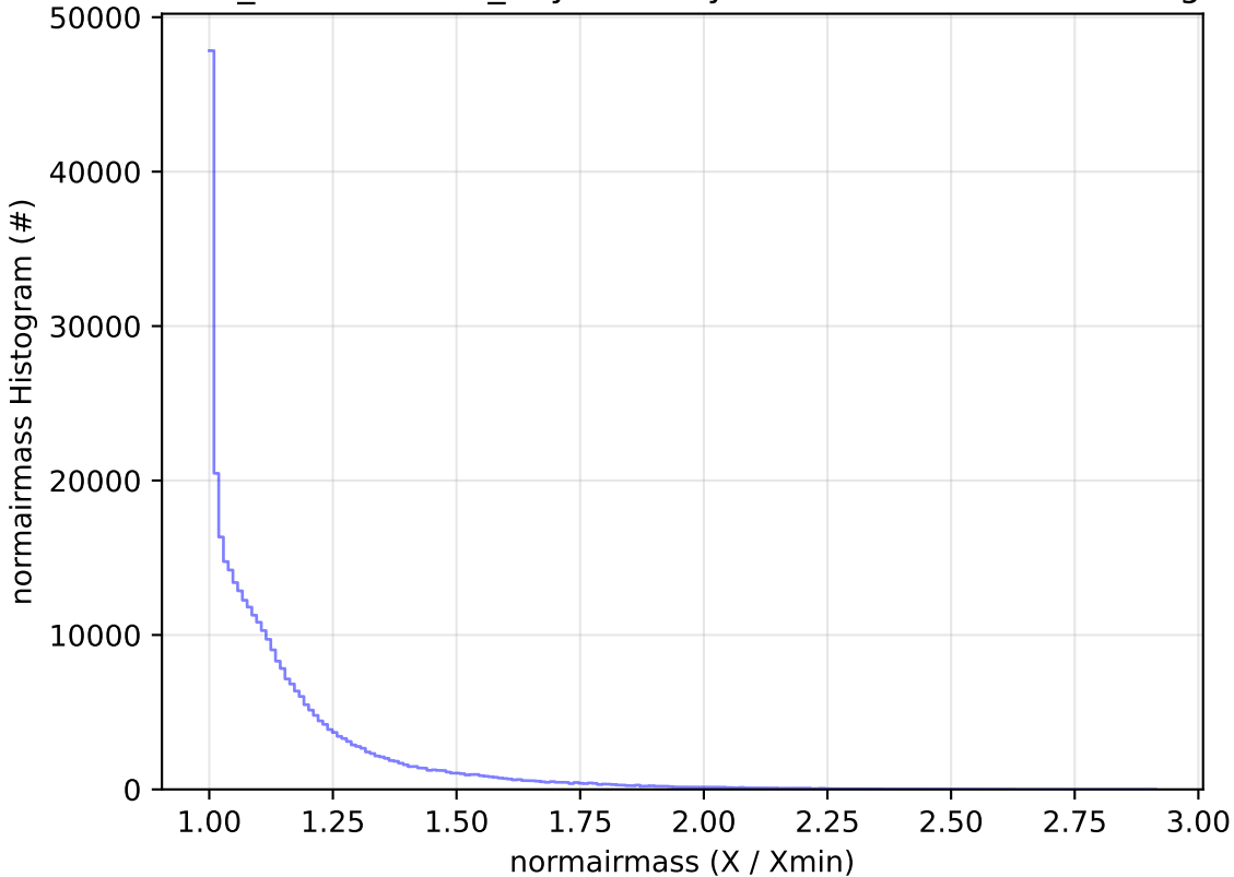
weather_cloudso0v3.5_10yrs WFD y band: normairmass Histogram
