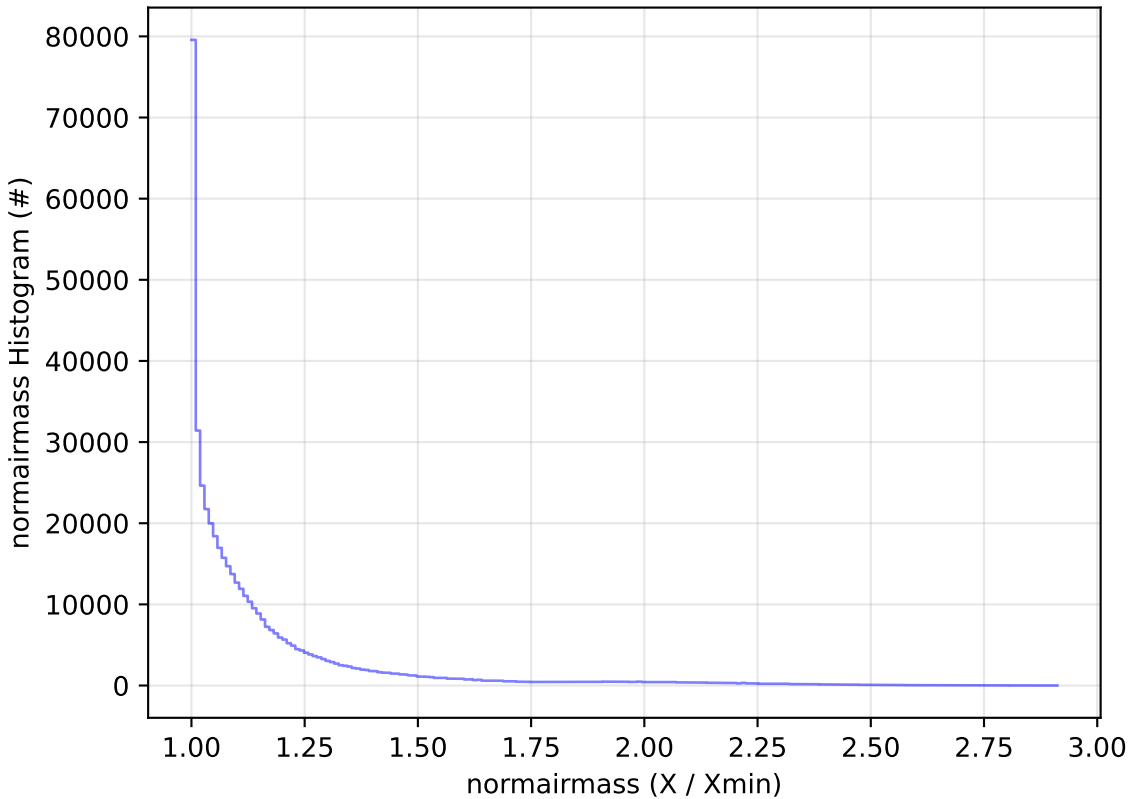
weather_cloudso0v3.5_10yrs WFD r band: normairmass Histogram
