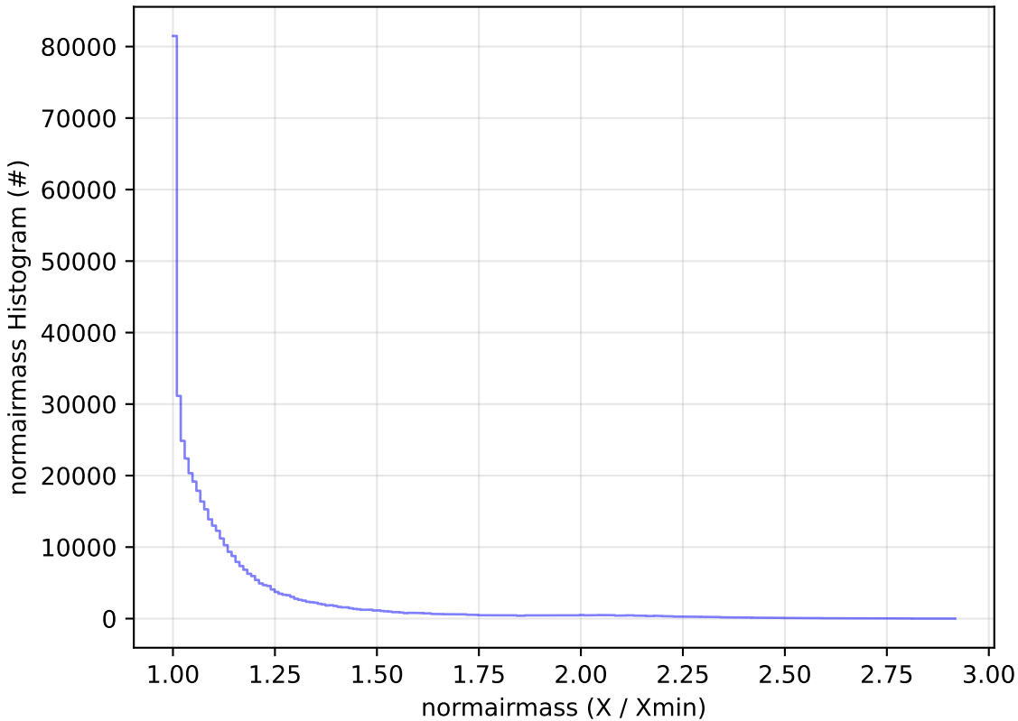
weather_cloudso0v3.5_10yrs WFD i band: normairmass Histogram
