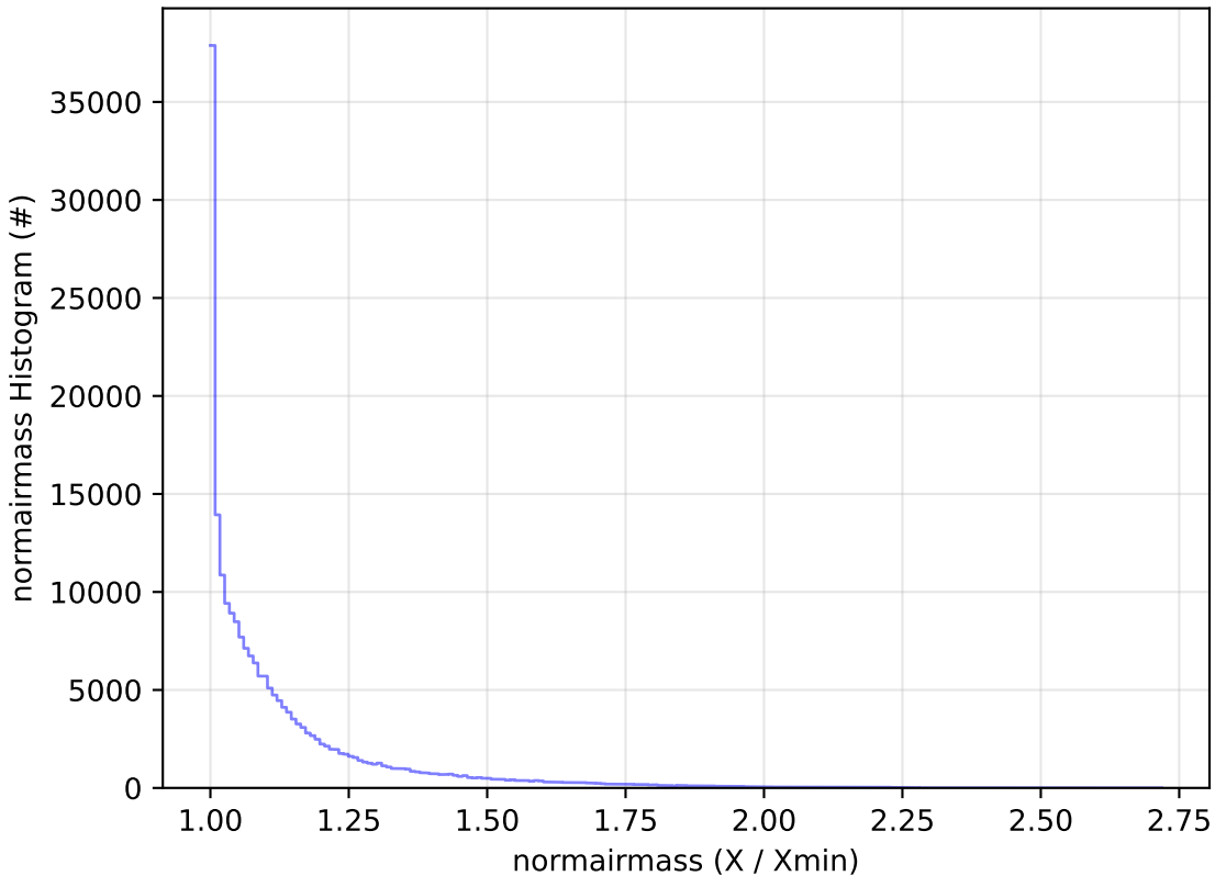
weather_cloudso0v3.5_10yrs WFD g band: normairmass Histogram
