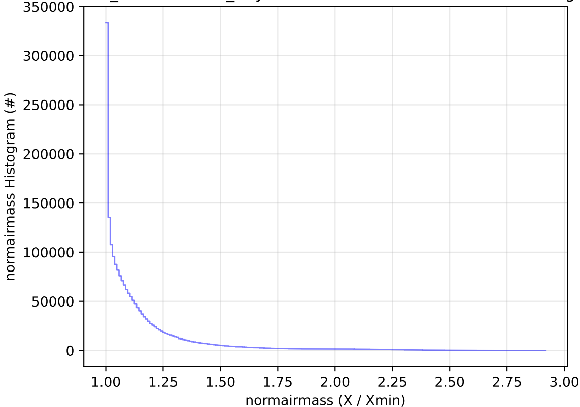
weather_cloudso0v3.5_10yrs WFD all bands: normairmass Histogram
