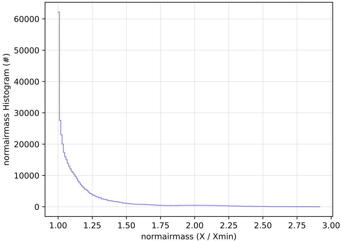
weather_cloudso0v3.5_10yrs All sky z band: normairmass Histogram
