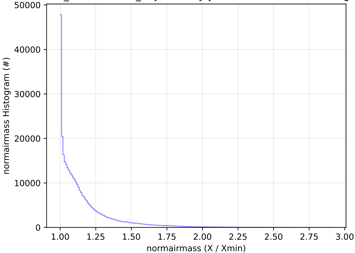
weather_cloudso0v3.5_10yrs All sky y band: normairmass Histogram
