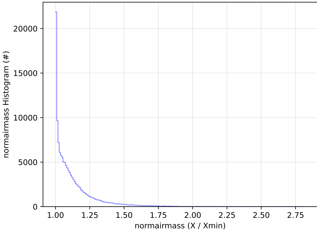
weather_cloudso0v3.5_10yrs All sky u band: normairmass Histogram
