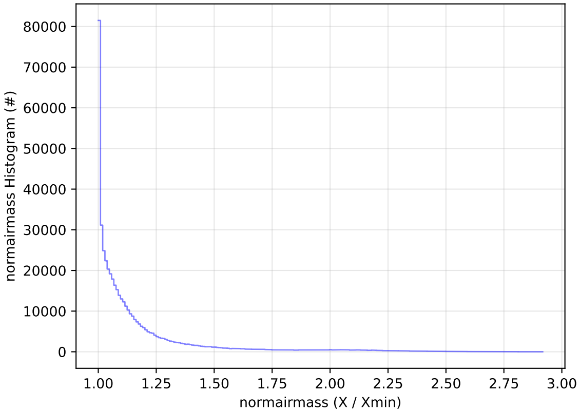
weather_cloudso0v3.5_10yrs All sky i band: normairmass Histogram
