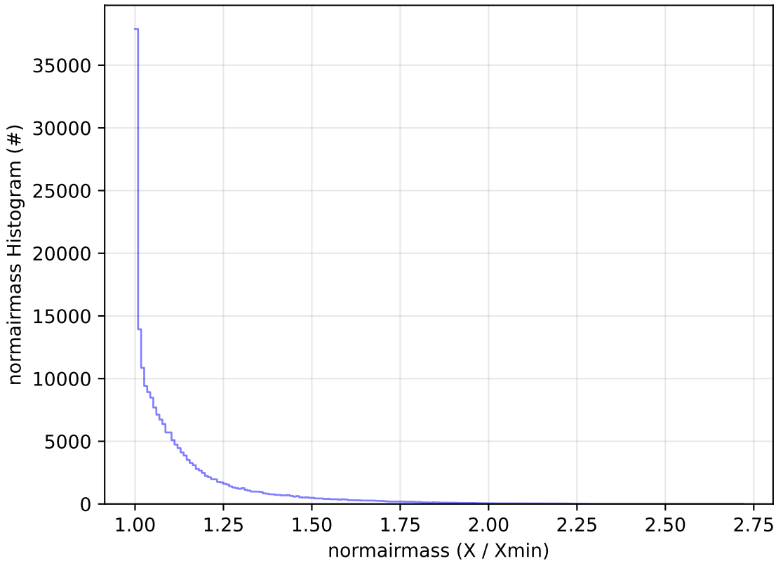
weather_cloudso0v3.5_10yrs All sky g band: normairmass Histogram
