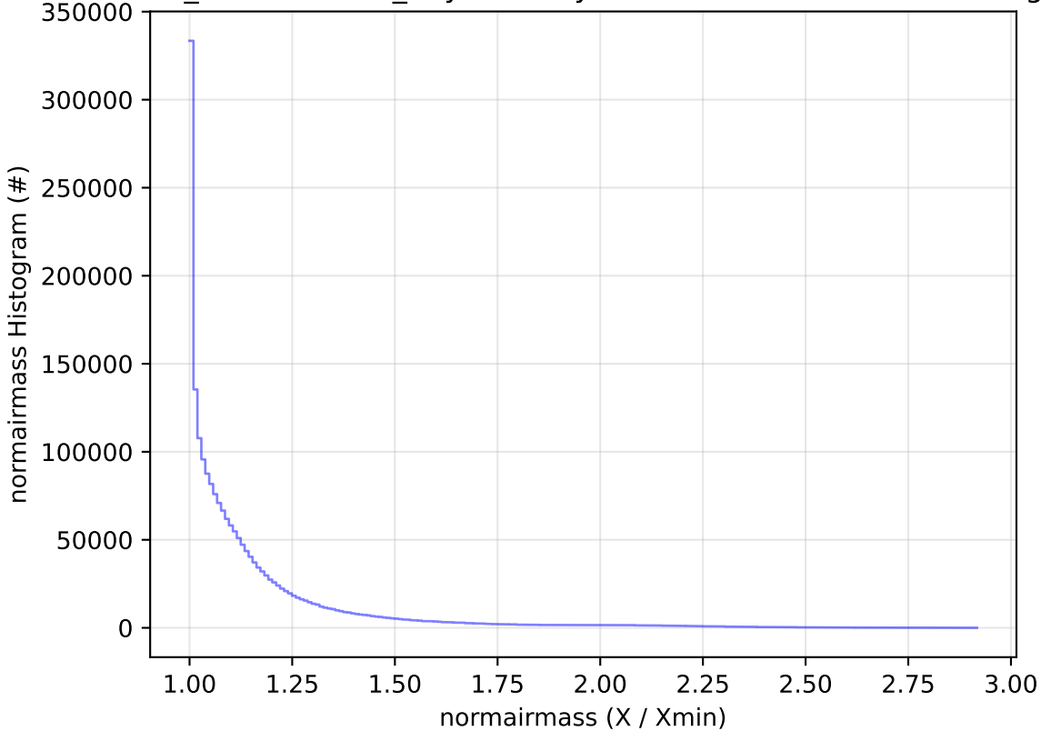
weather_cloudso0v3.5_10yrs All sky all bands: normairmass Histogram
