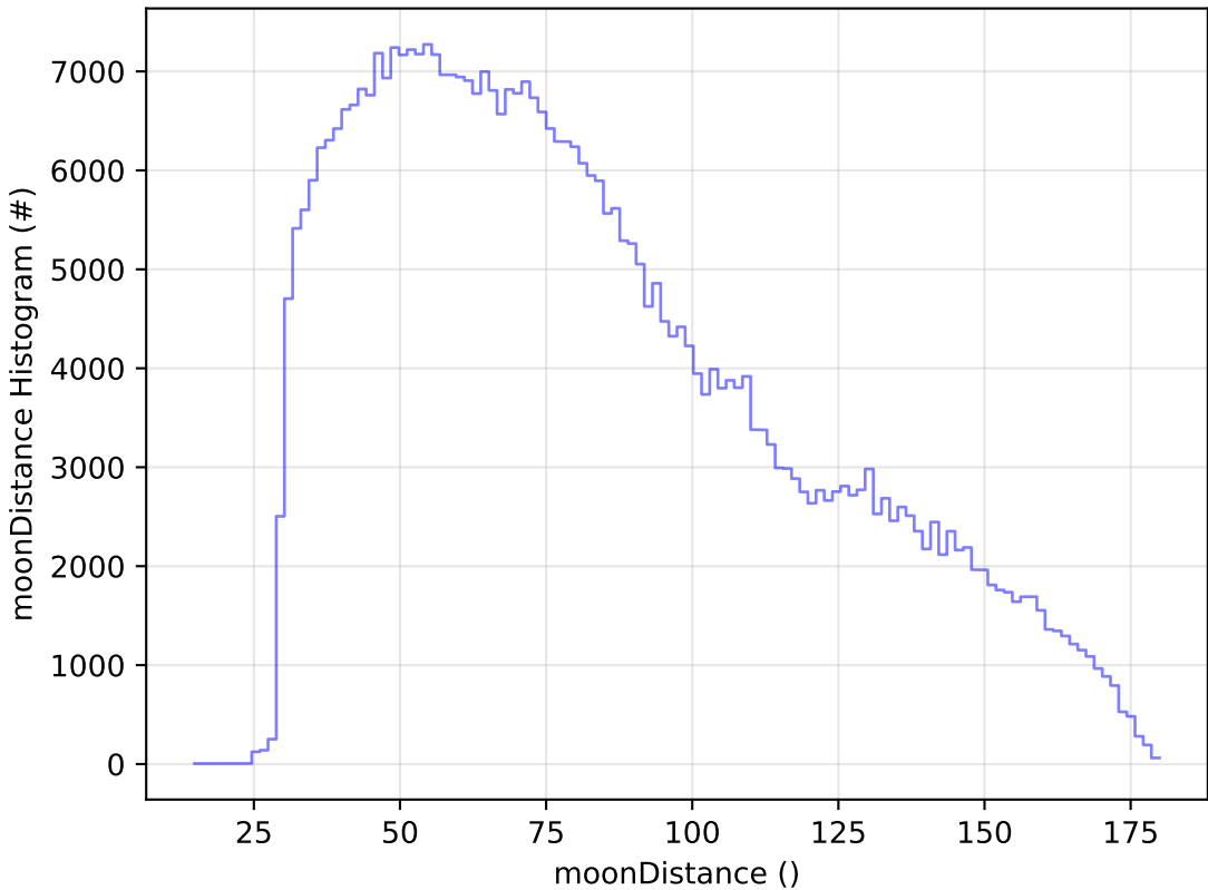
weather_cloudso0v3.5_10yrs WFD z band: moonDistance Histogram
