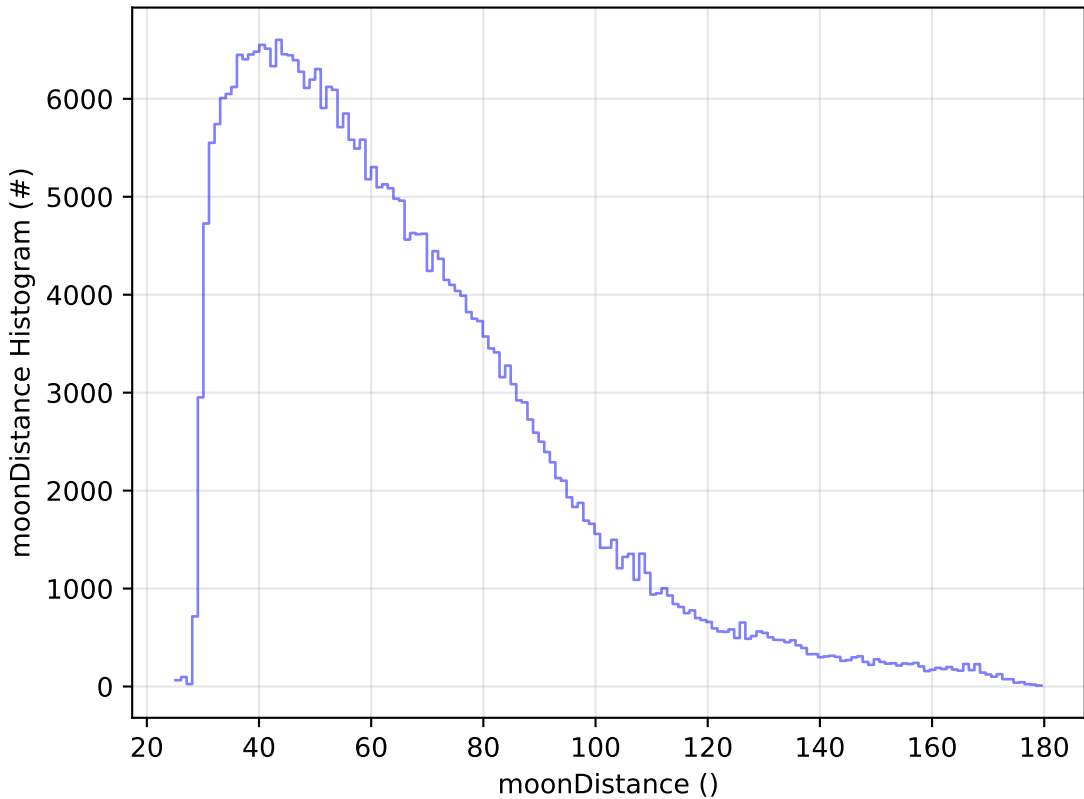
weather_cloudso0v3.5_10yrs WFD y band: moonDistance Histogram
