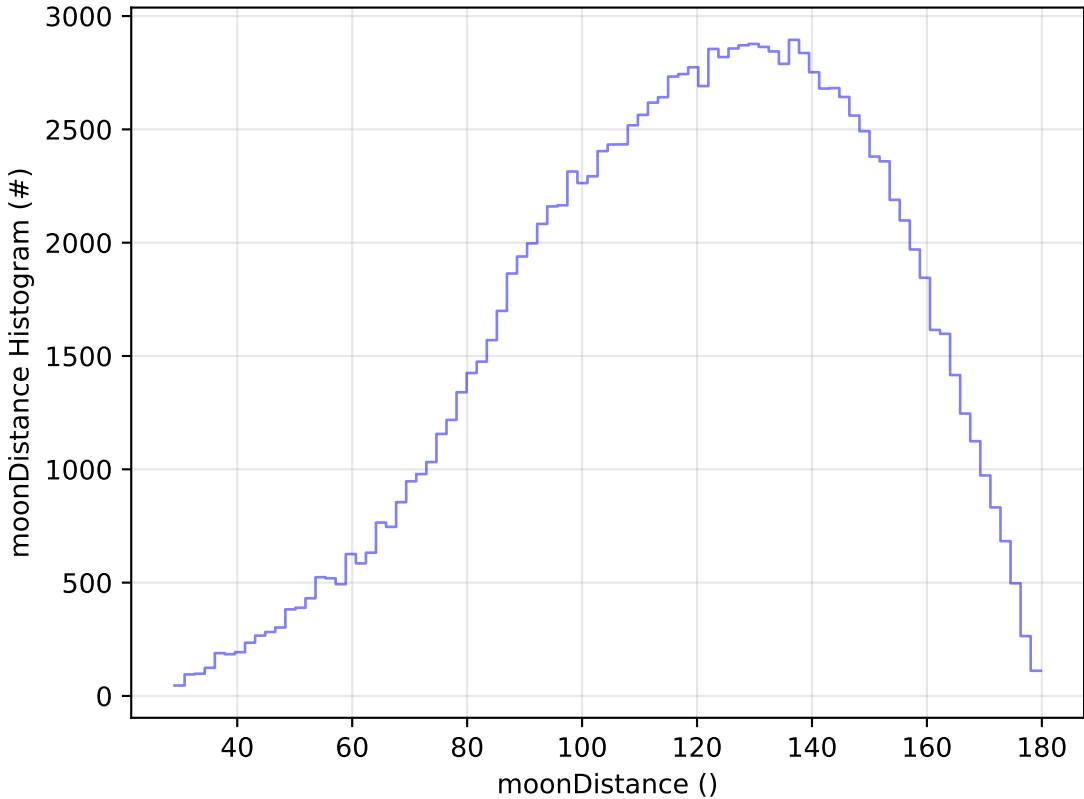
weather_cloudso0v3.5_10yrs WFD u band: moonDistance Histogram
