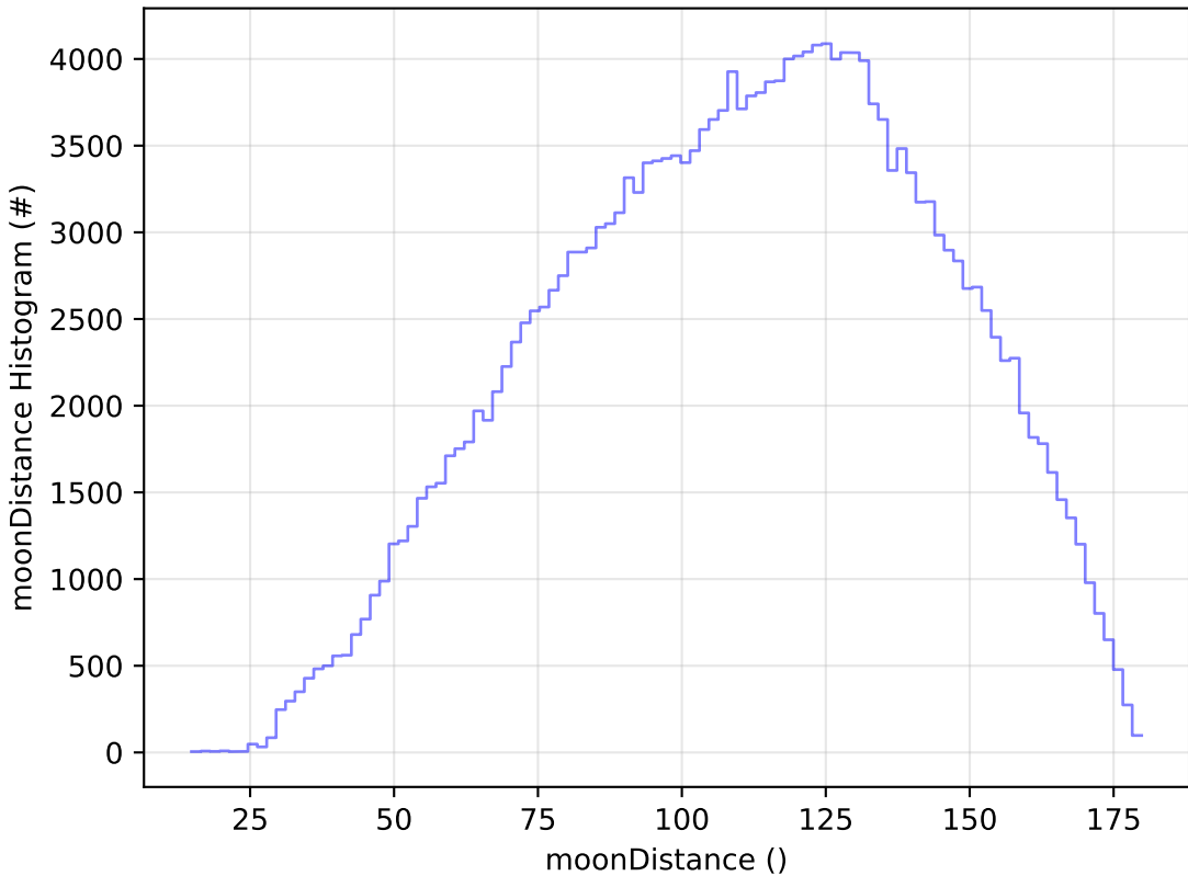
weather_cloudso0v3.5_10yrs WFD g band: moonDistance Histogram
