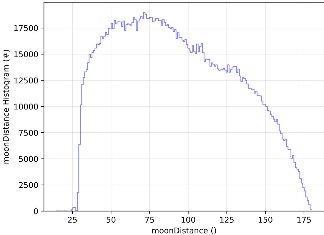
weather_cloudso0v3.5_10yrs WFD all bands: moonDistance Histogram
