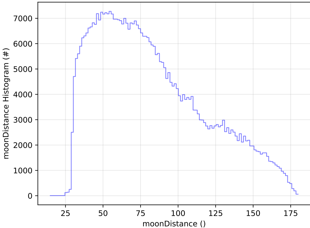
weather_cloudso0v3.5_10yrs All sky z band: moonDistance Histogram
