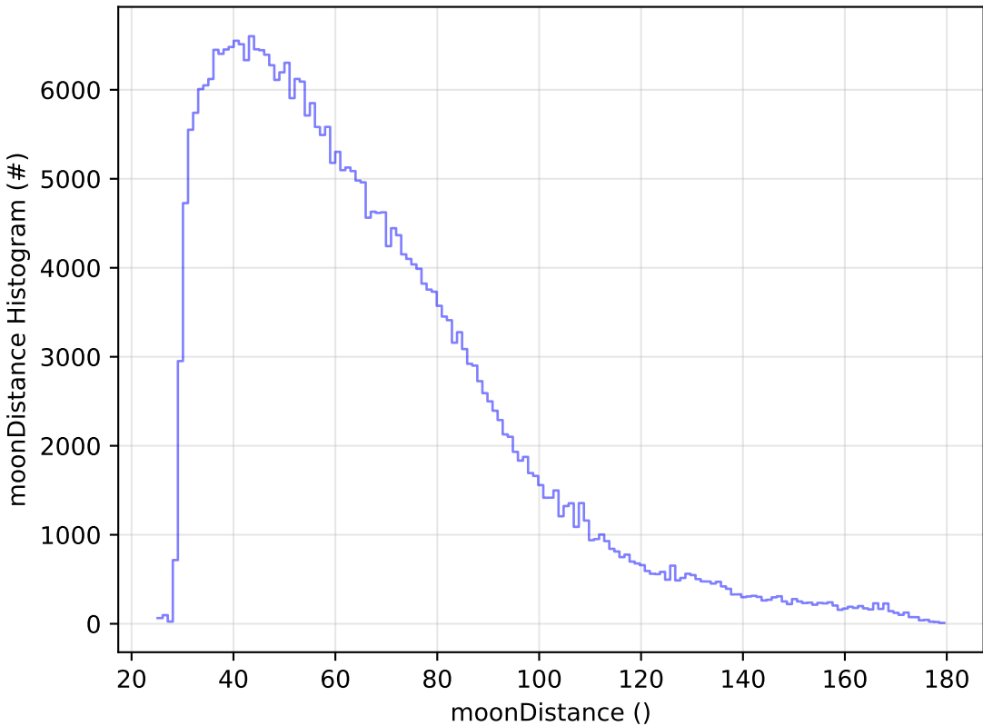
weather_cloudso0v3.5_10yrs All sky y band: moonDistance Histogram
