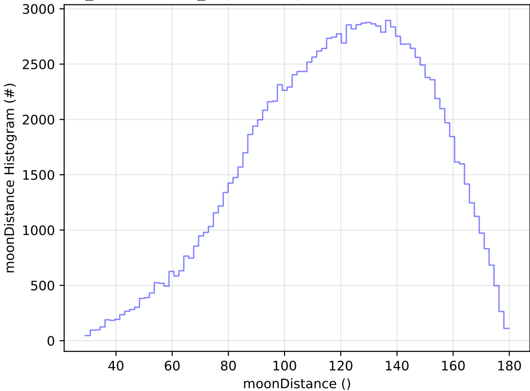
weather_cloudso0v3.5_10yrs All sky u band: moonDistance Histogram
