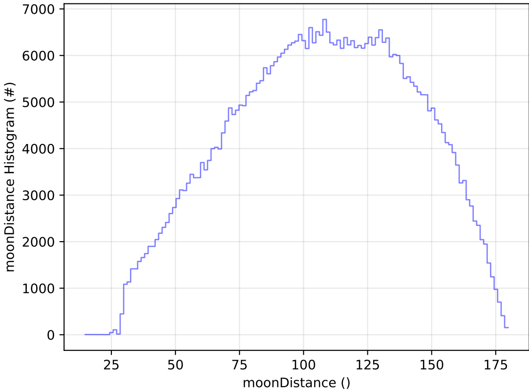
weather_cloudso0v3.5_10yrs All sky r band: moonDistance Histogram
