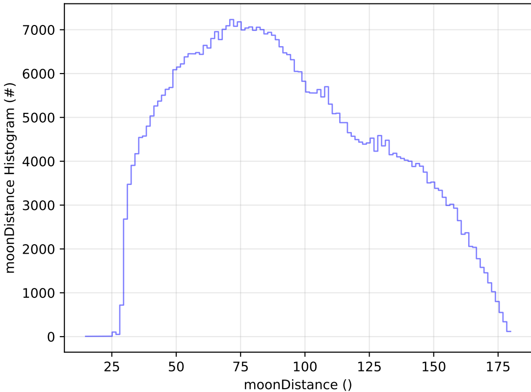
weather_cloudso0v3.5_10yrs All sky i band: moonDistance Histogram
