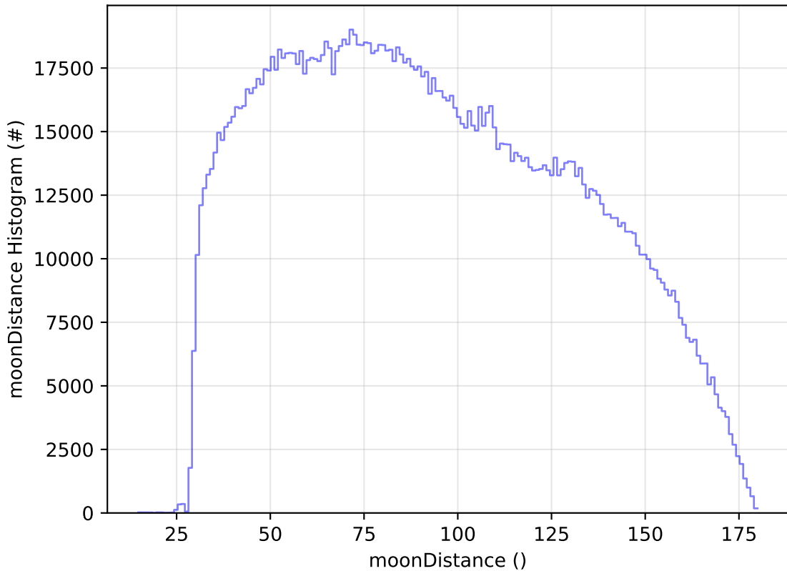
weather_cloudso0v3.5_10yrs All sky all bands: moonDistance Histogram
