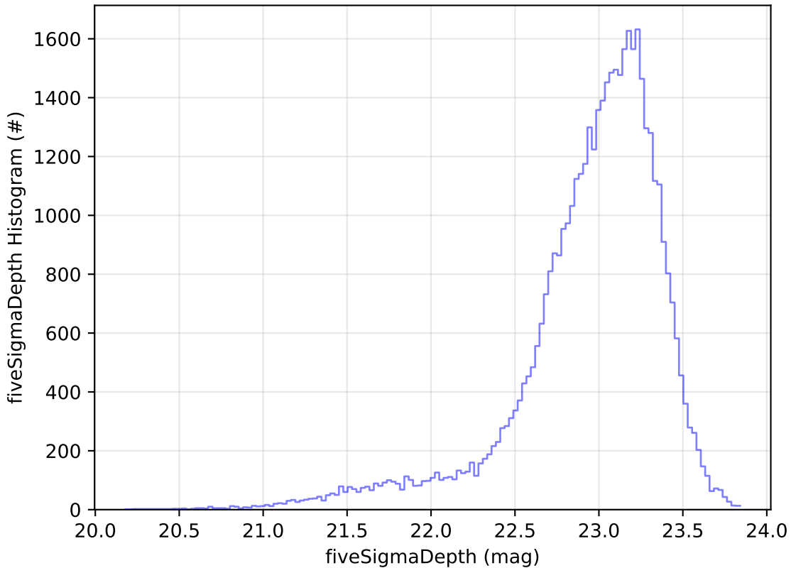
weather_cloudso0v3.5_10yrs Yr 1 z band: fiveSigmaDepth Histogram
