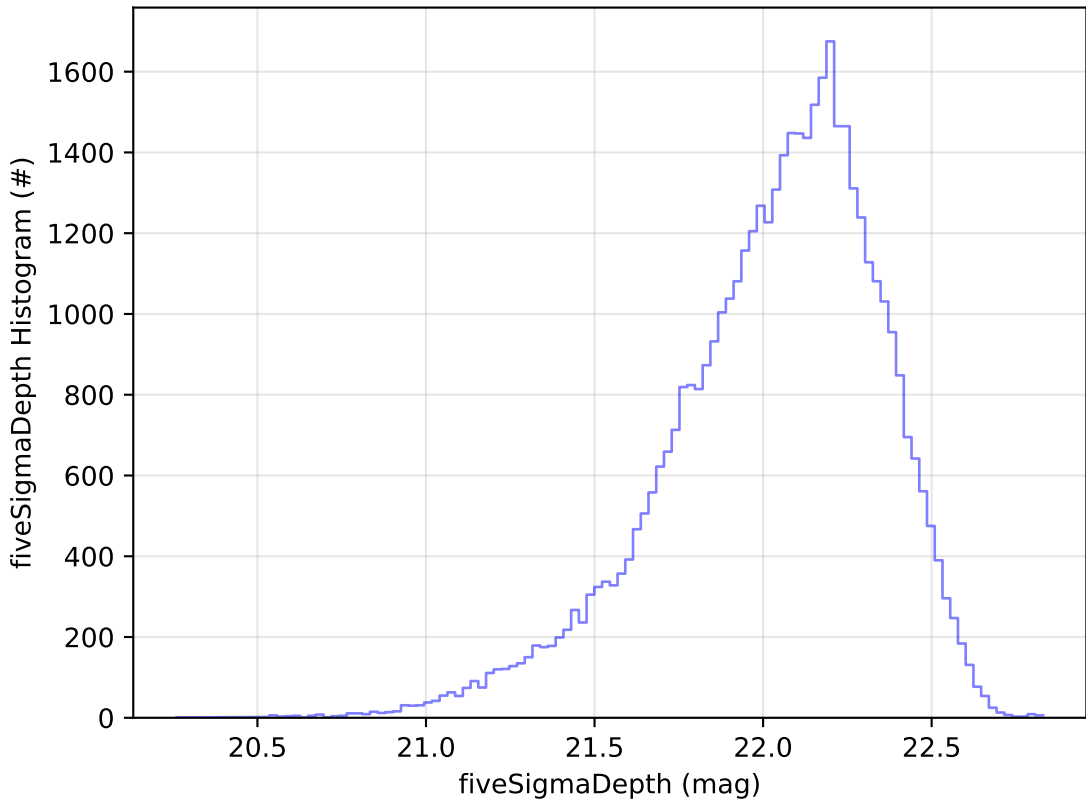
weather_cloudso0v3.5_10yrs Yr 1 y band: fiveSigmaDepth Histogram
