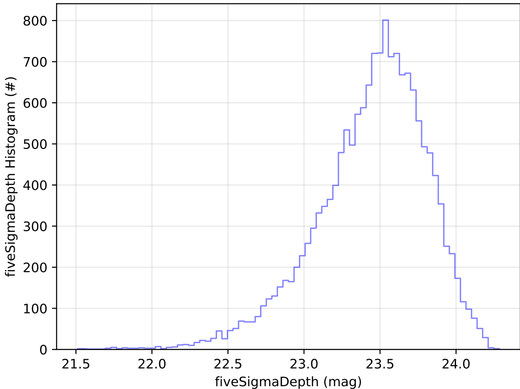
weather_cloudso0v3.5_10yrs Yr 1 u band: fiveSigmaDepth Histogram
