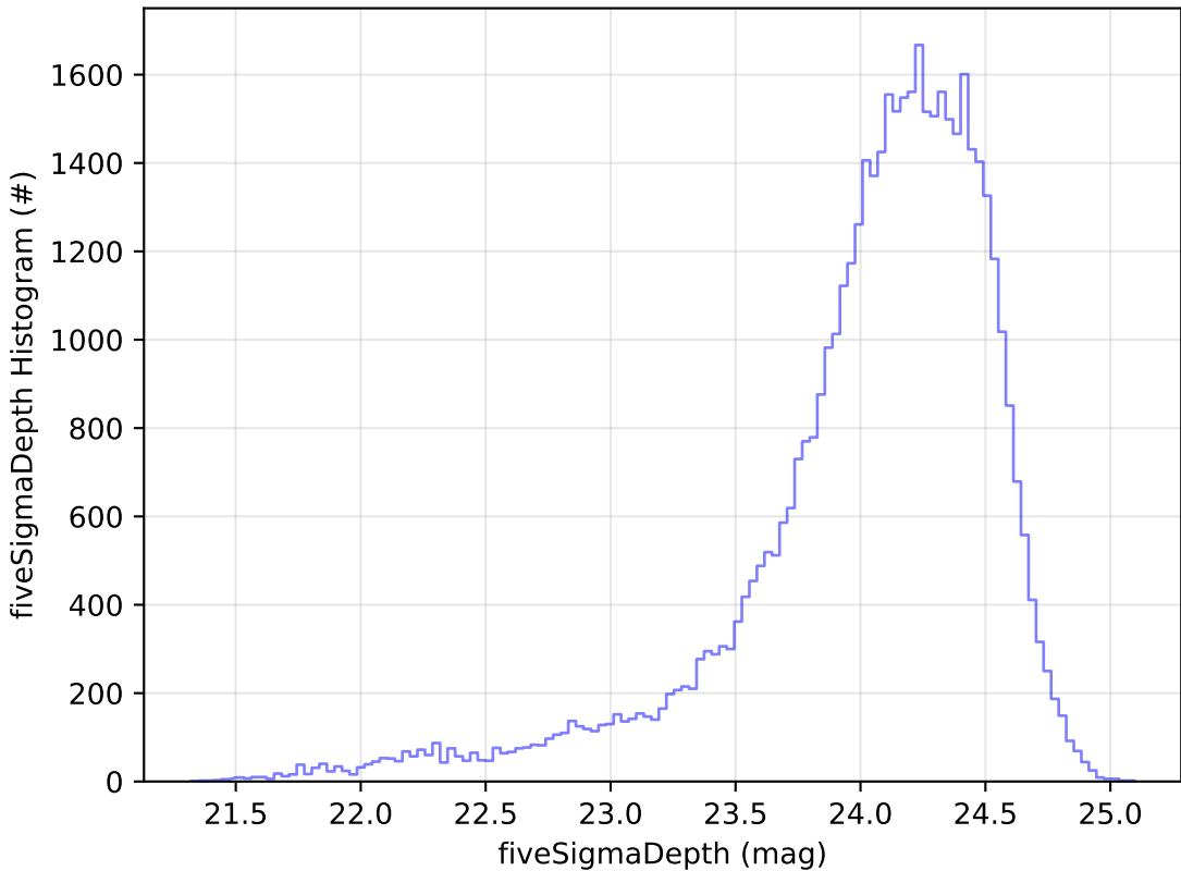
weather_cloudso0v3.5_10yrs Yr 1 r band: fiveSigmaDepth Histogram
