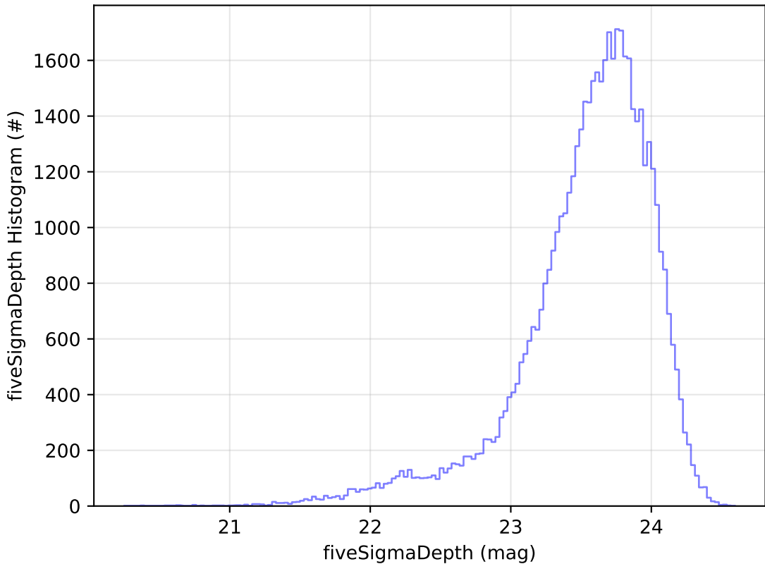
weather_cloudso0v3.5_10yrs Yr 1 i band: fiveSigmaDepth Histogram
