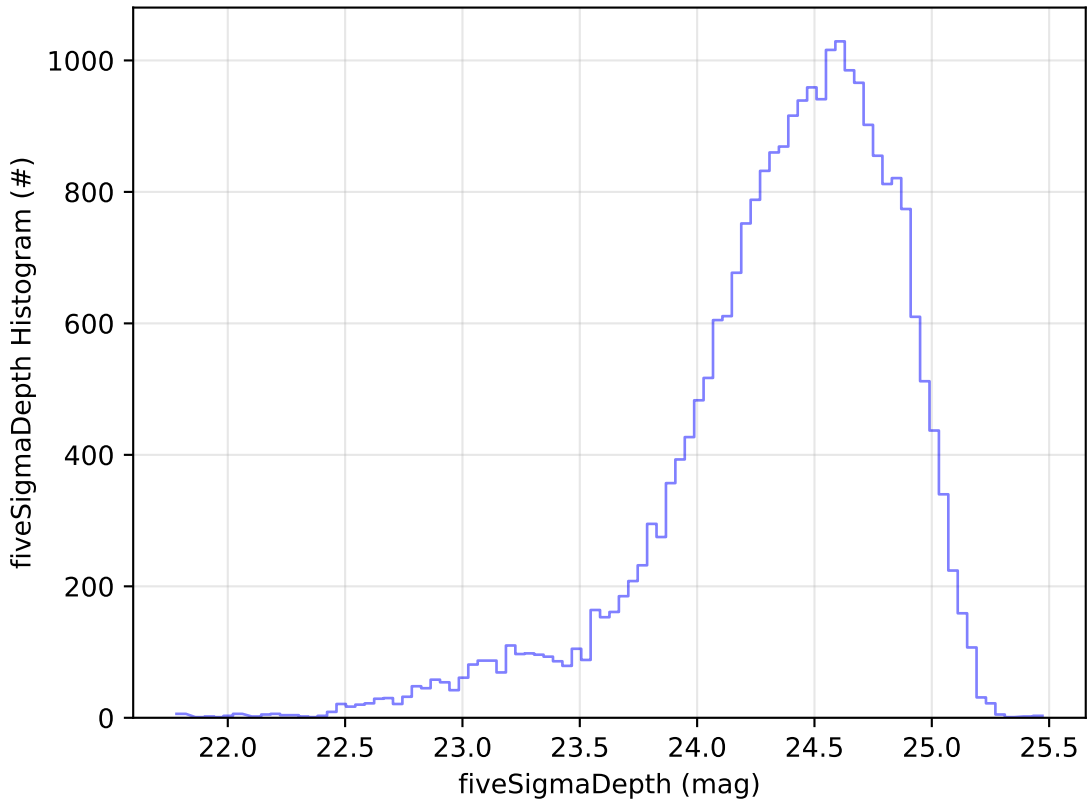
weather_cloudso0v3.5_10yrs Yr 1 g band: fiveSigmaDepth Histogram
