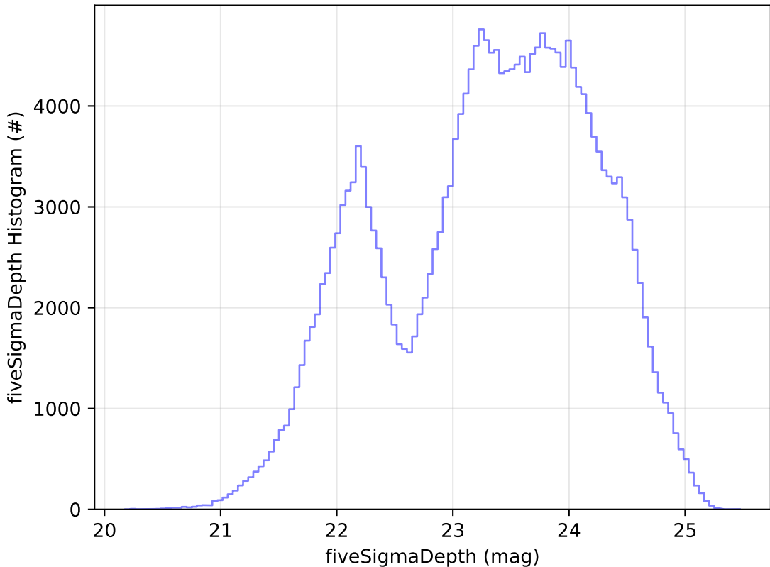
weather_cloudso0v3.5_10yrs Yr 1 all bands: fiveSigmaDepth Histogram
