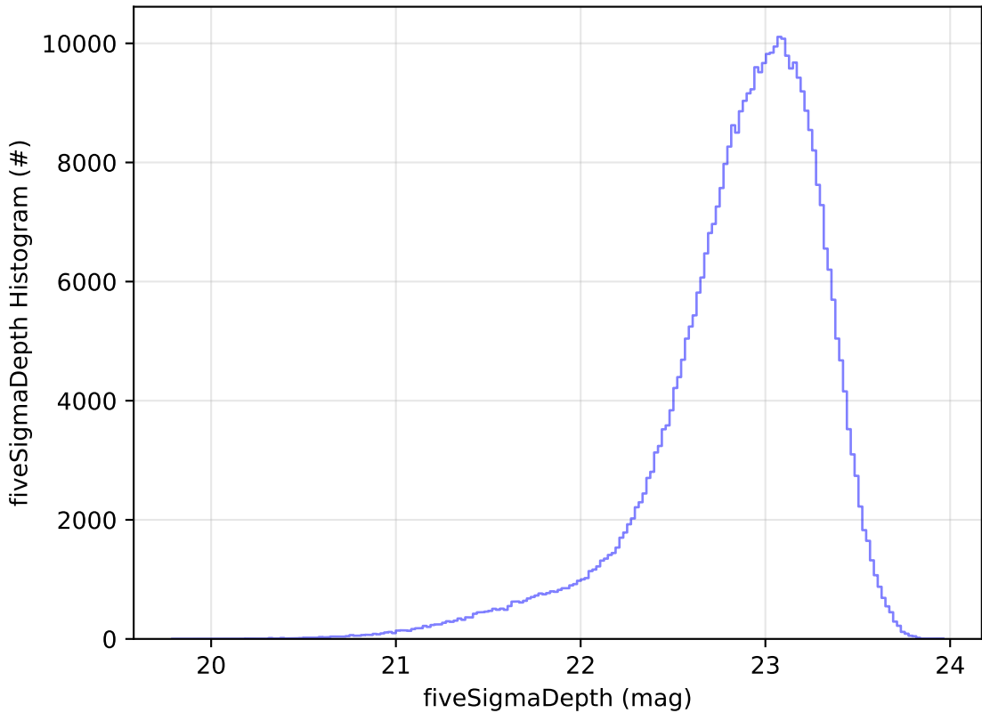
weather_cloudso0v3.5_10yrs WFD z band: fiveSigmaDepth Histogram
