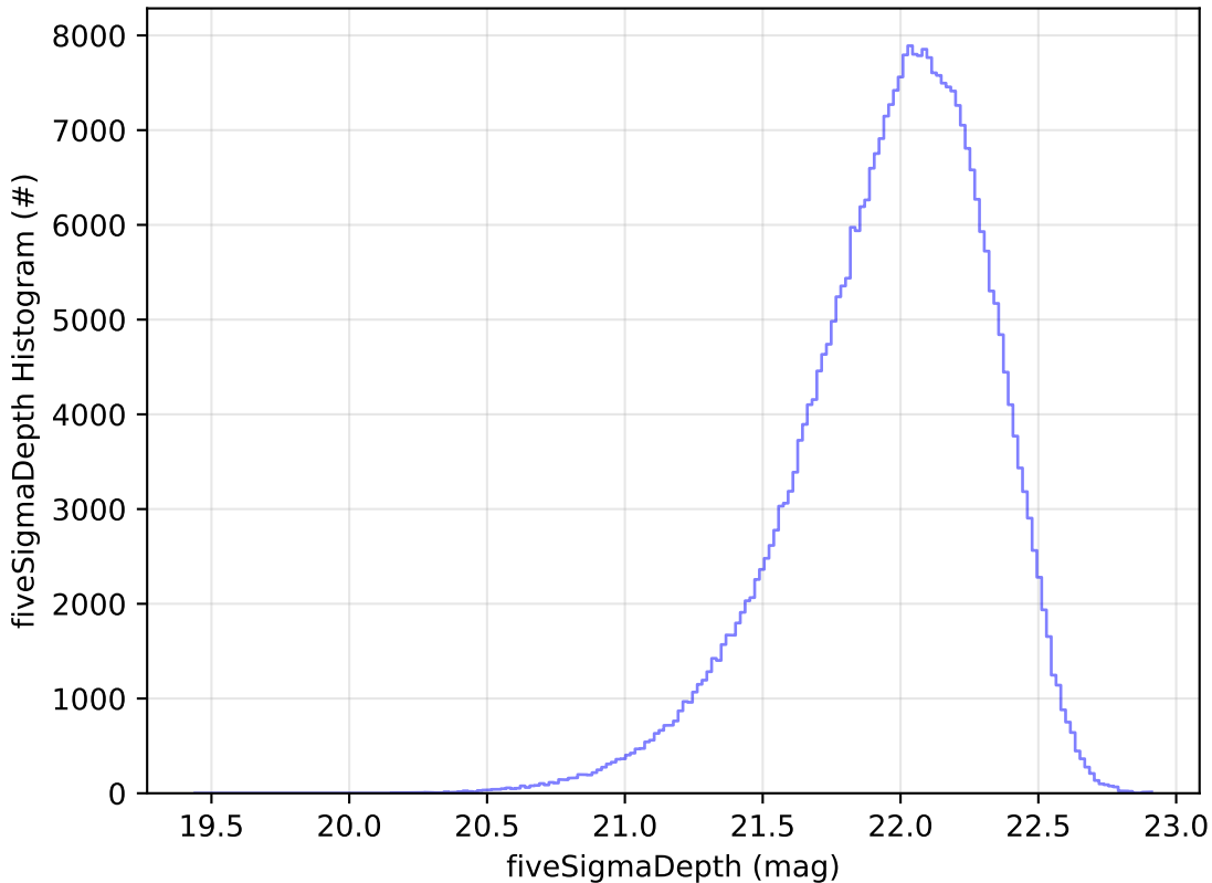
weather_cloudso0v3.5_10yrs WFD y band: fiveSigmaDepth Histogram
