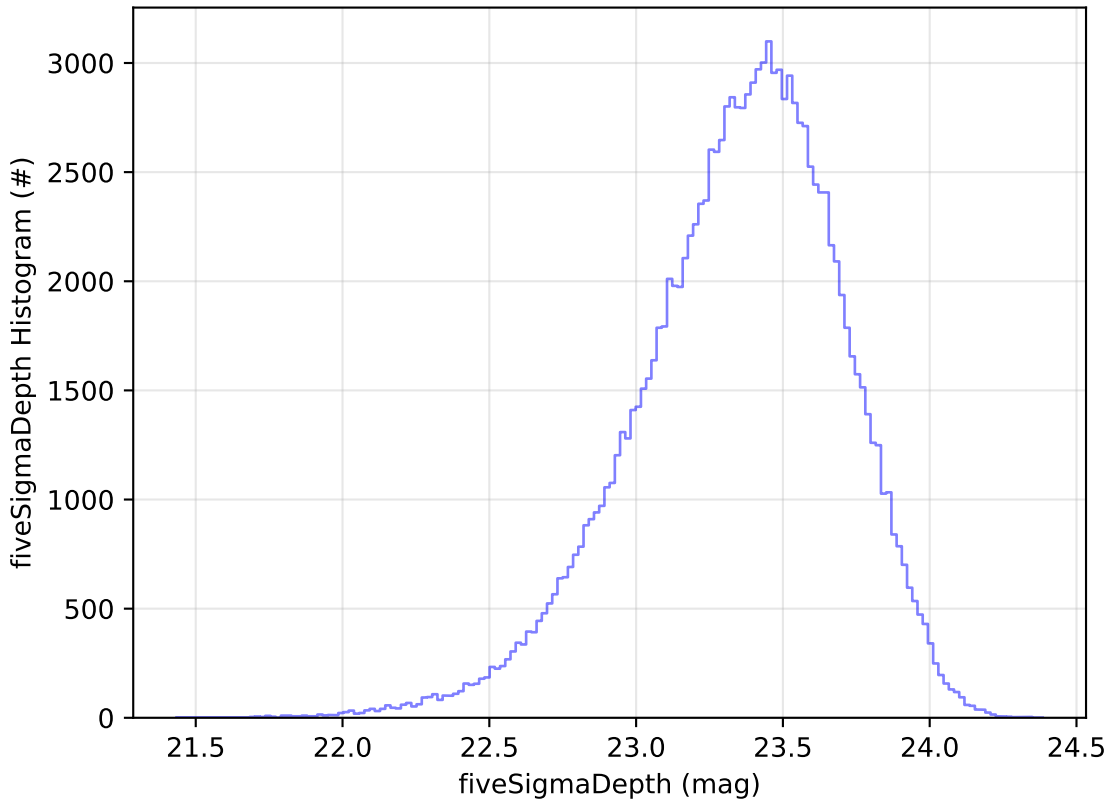
weather_cloudso0v3.5_10yrs WFD u band: fiveSigmaDepth Histogram
