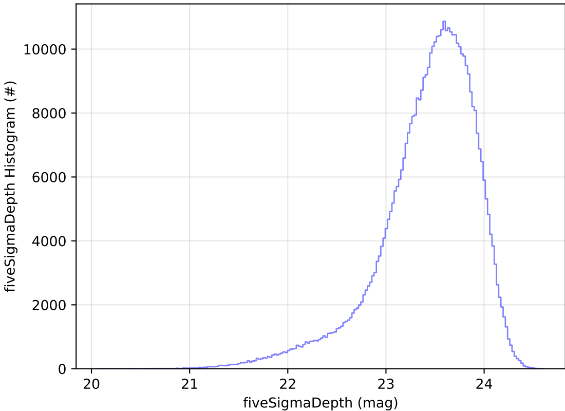
weather_cloudso0v3.5_10yrs WFD i band: fiveSigmaDepth Histogram
