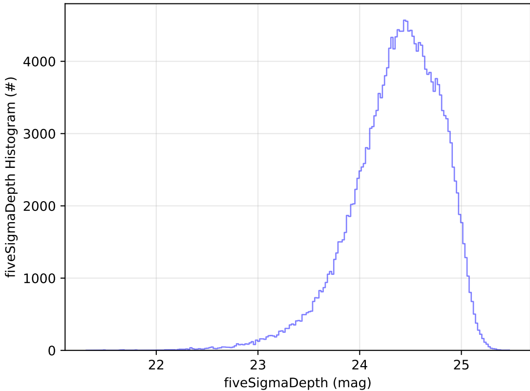
weather_cloudso0v3.5_10yrs WFD g band: fiveSigmaDepth Histogram
