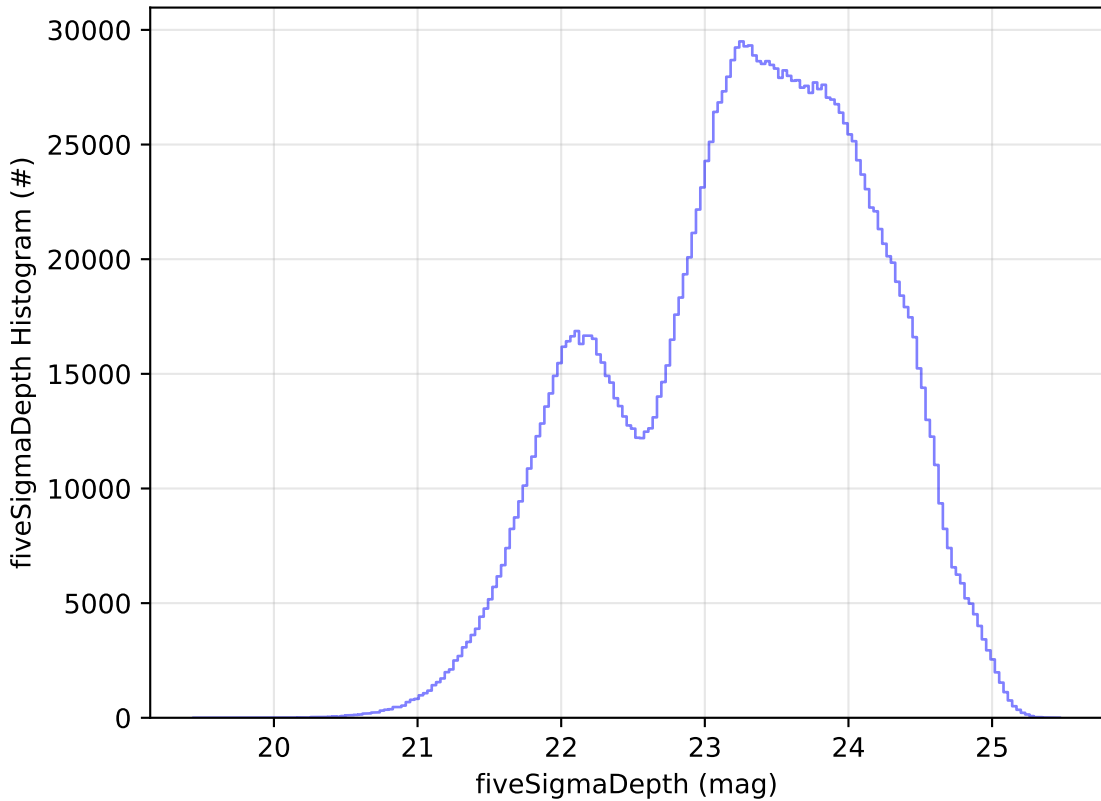
weather_cloudso0v3.5_10yrs WFD all bands: fiveSigmaDepth Histogram
