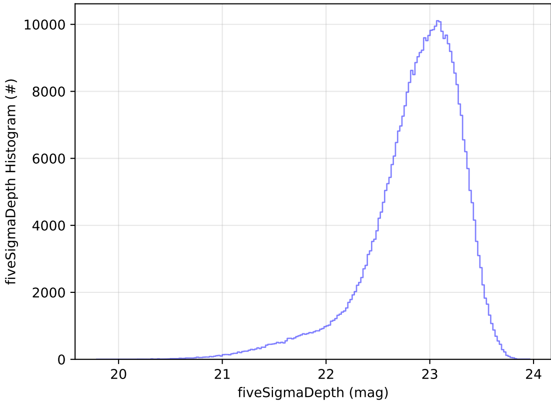
weather_cloudso0v3.5_10yrs All sky z band: fiveSigmaDepth Histogram
