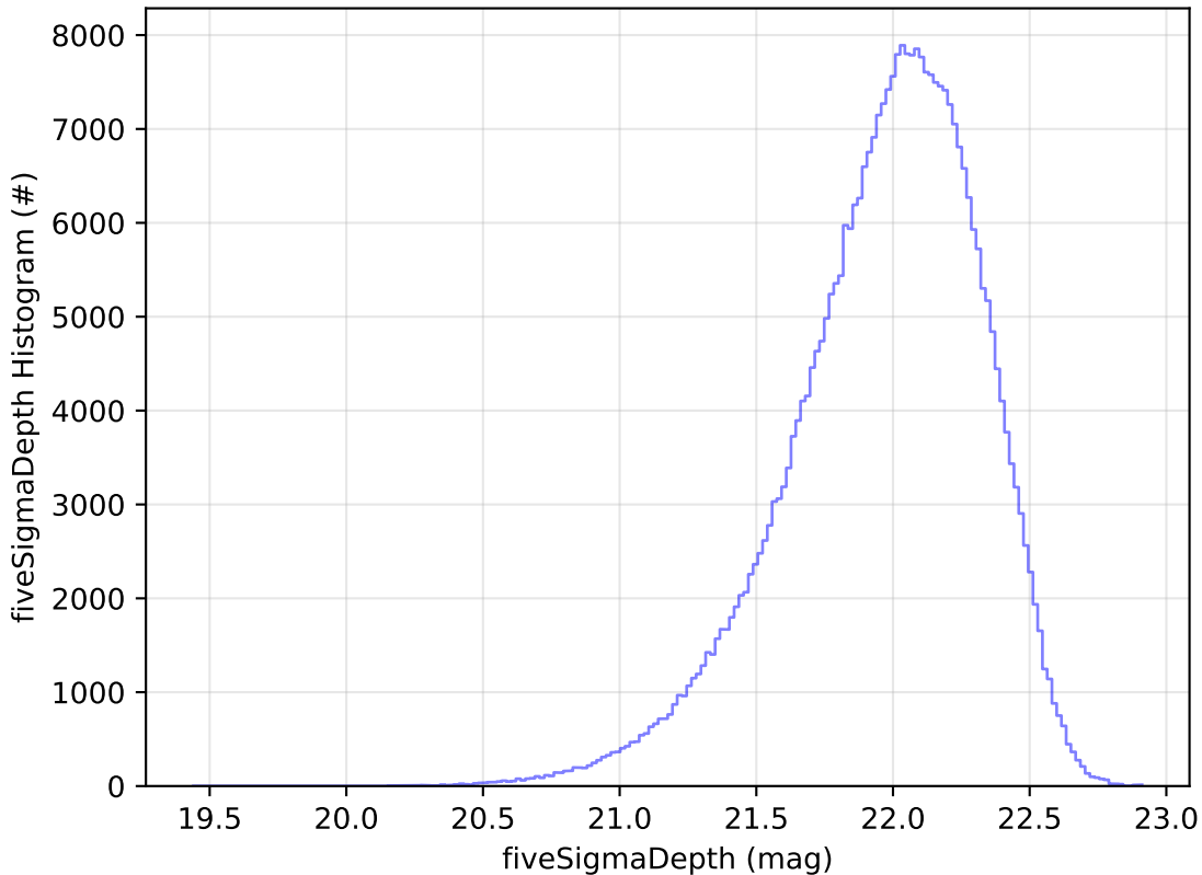
weather_cloudso0v3.5_10yrs All sky y band: fiveSigmaDepth Histogram
