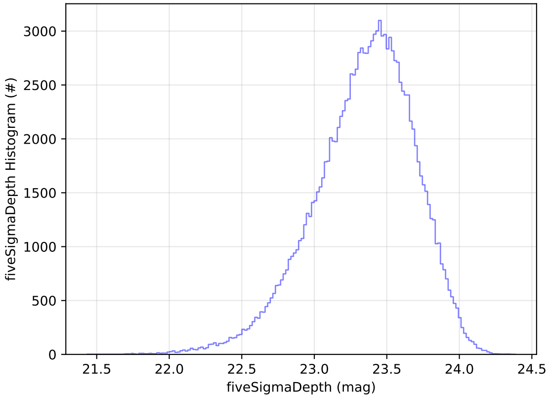
weather_cloudso0v3.5_10yrs All sky u band: fiveSigmaDepth Histogram
