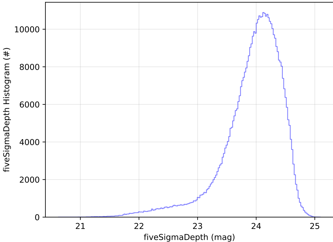
weather_cloudso0v3.5_10yrs All sky r band: fiveSigmaDepth Histogram
