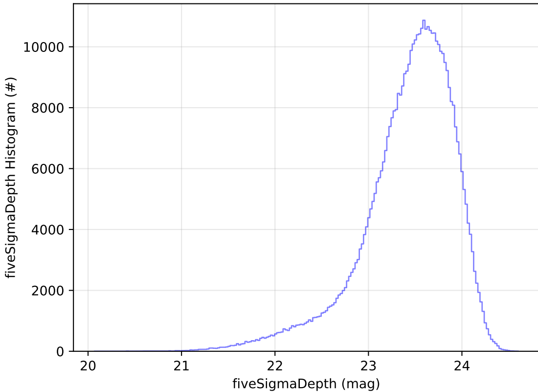
weather_cloudso0v3.5_10yrs All sky i band: fiveSigmaDepth Histogram
