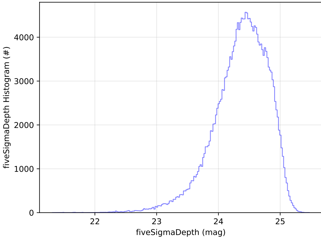
weather_cloudso0v3.5_10yrs All sky g band: fiveSigmaDepth Histogram
