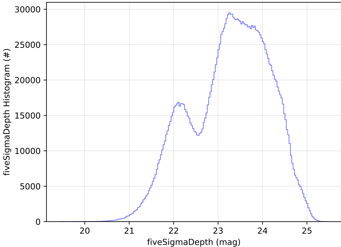
weather_cloudso0v3.5_10yrs All sky all bands: fiveSigmaDepth Histogram
